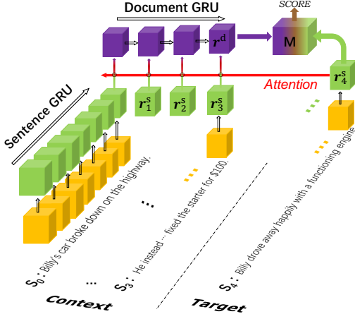
Figure 2: Discriminator Network. Yellow blocks denote word embedding, green and purple blocks stand for sentence and document GRU hidden states respectively.
